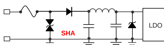
TVS The twice Stages Load Dump Protection Application for 24 V system (Due to Clamping Voltage issue)
