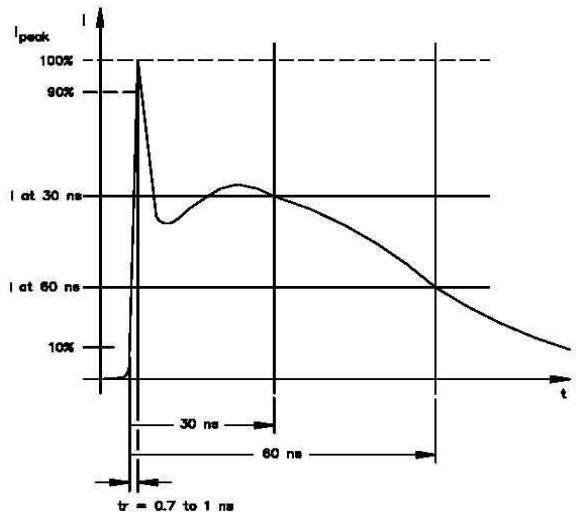
※ ESD protection waveform current
